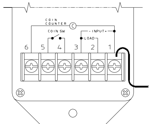
Wire is not used for 120VAC 120VAC CONNECTION
